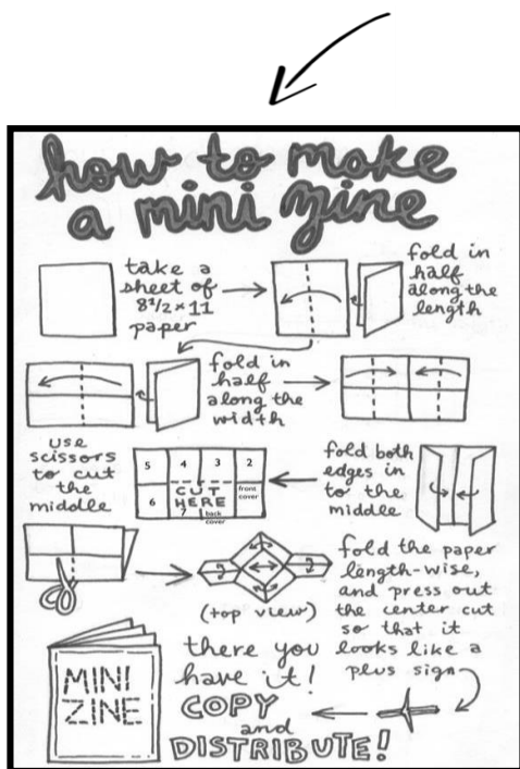
Figure 1. Simple fold 10
